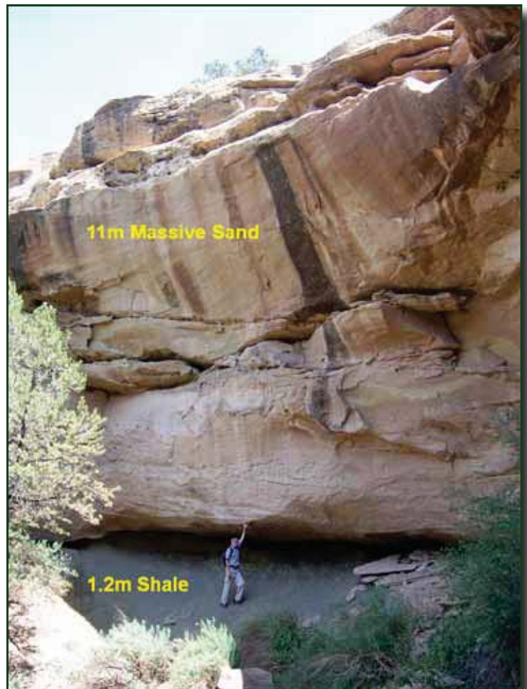
Figure 3. Massive sand that caps the site mesa. A weathered shale zone is observed at the base. Preferential erosion of the shale undercuts the sandstone layer.
